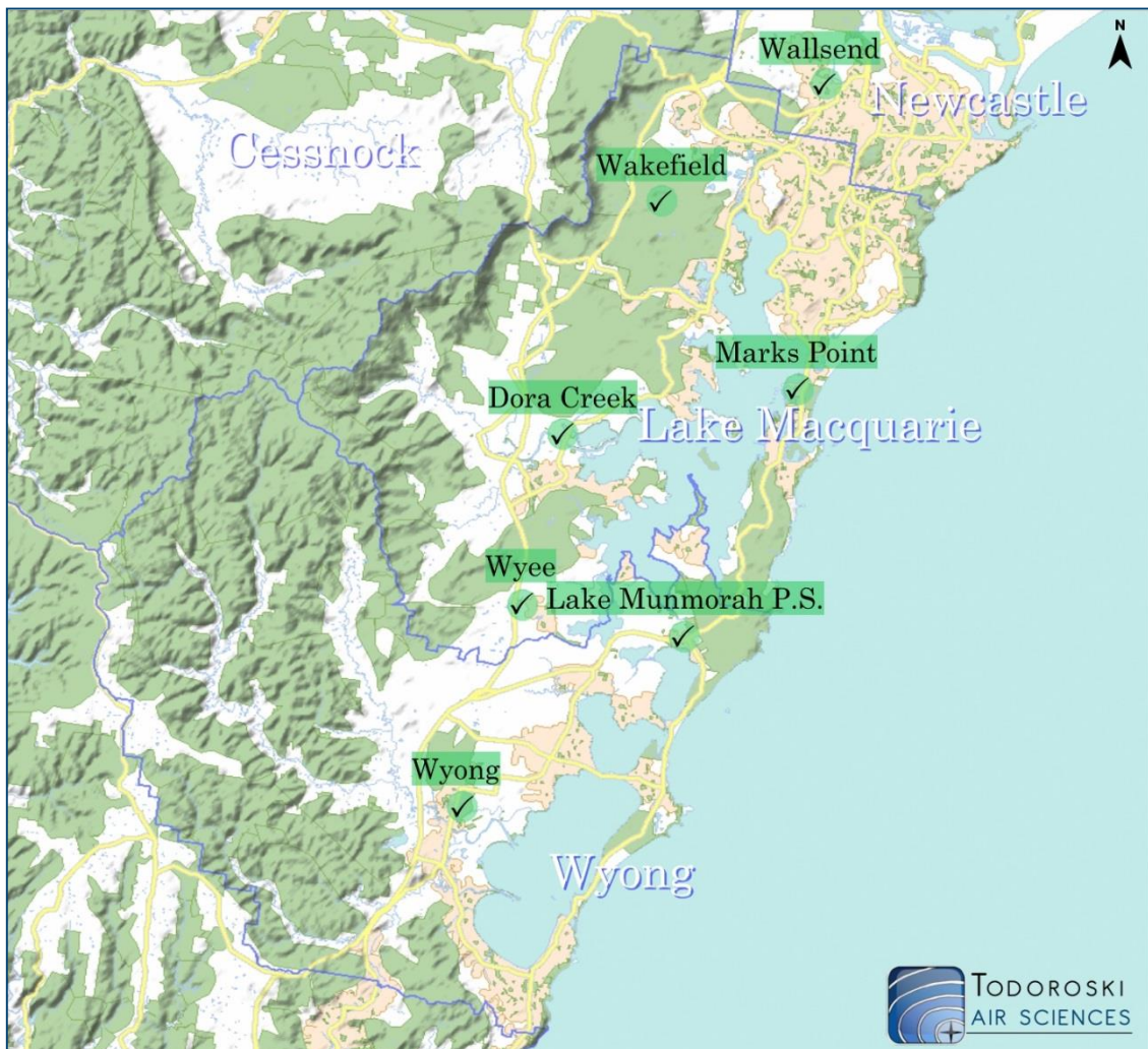
Lake Macquarie – Wyong Air Quality Tabular Summary - April 2014
