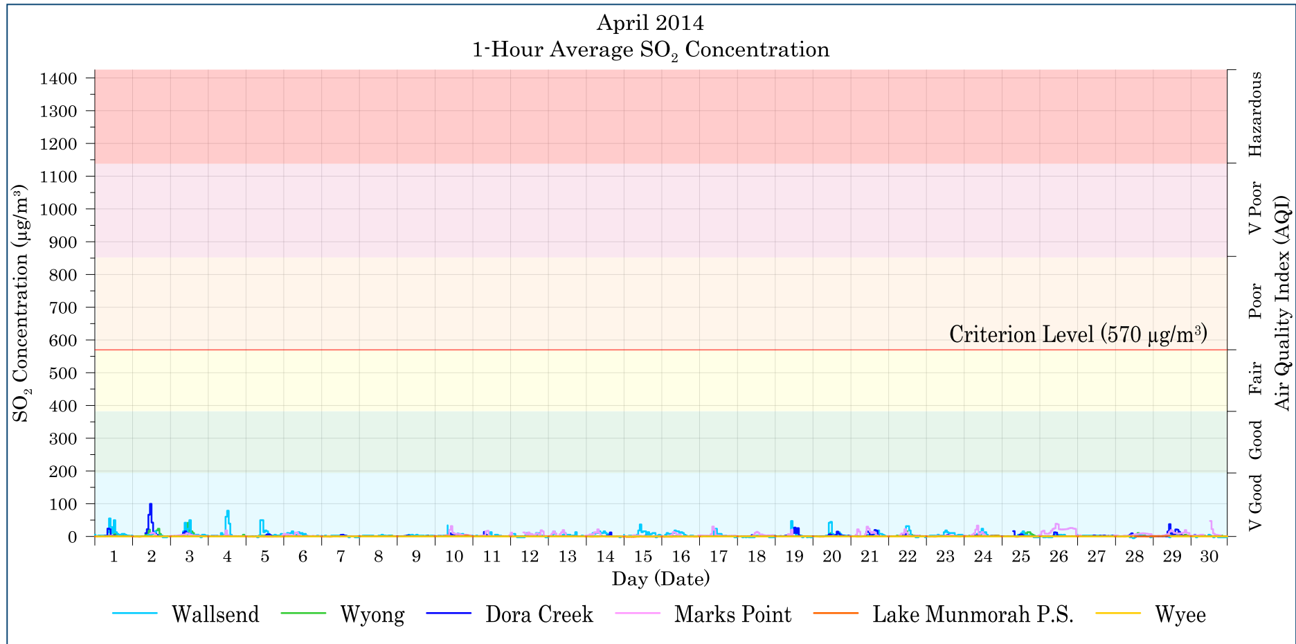
Figure 7-4: Lake Macquarie - Wyong 1-hour average SO 2 levels – April 2014
