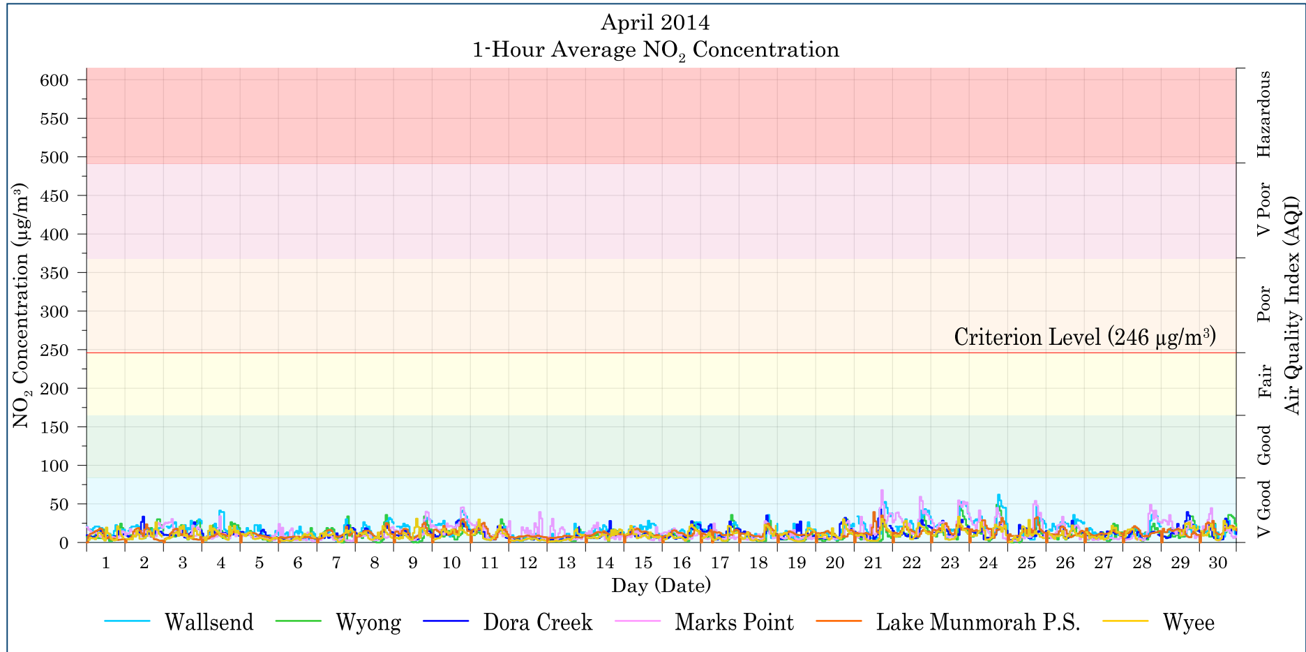
Figure 7-3: Lake Macquarie - Wyong 1-hour average NO 2 levels – April 2014
