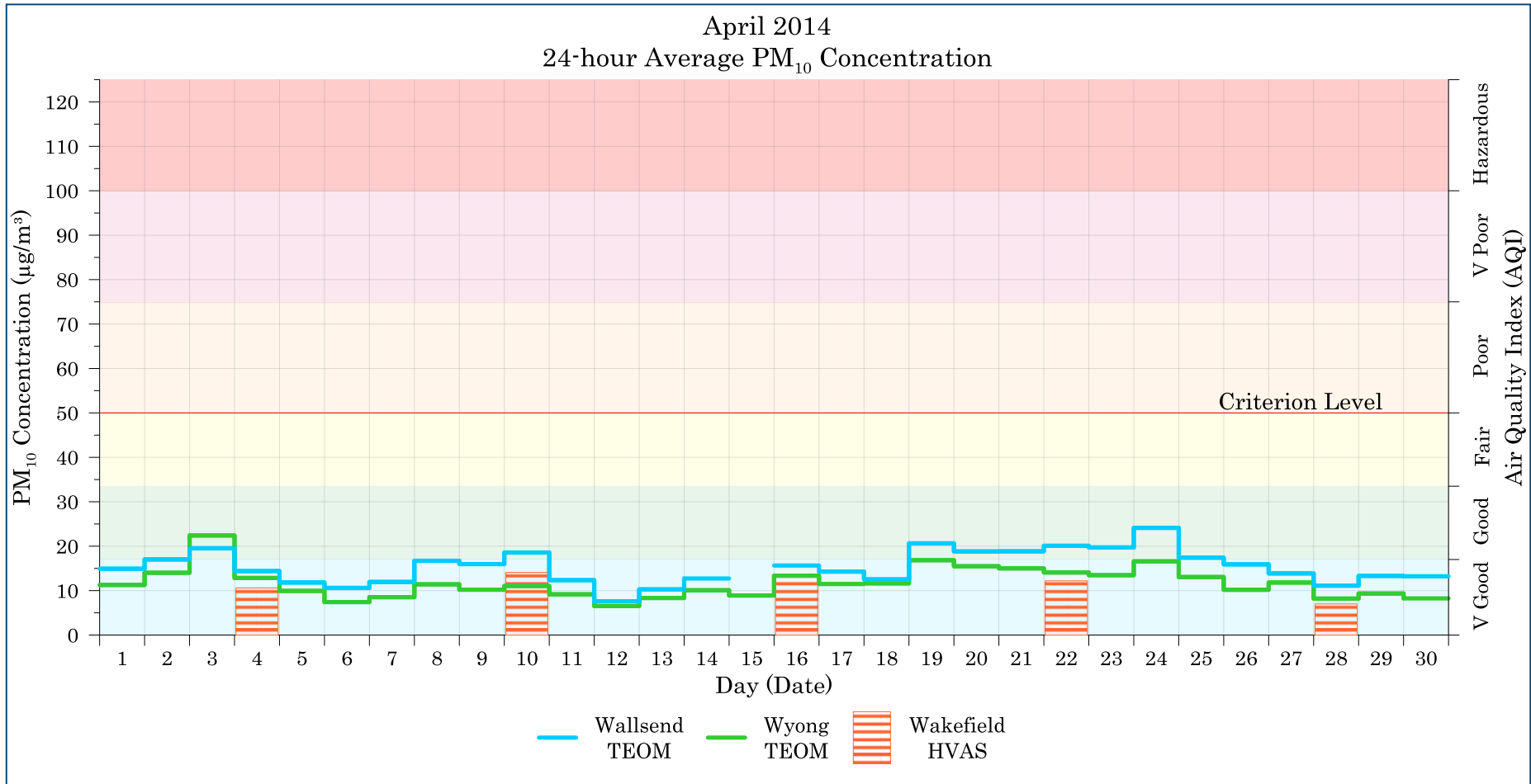
Figure 7-1: Lake Macquarie - Wyong 24-hour average PM 10 levels – April 2014
