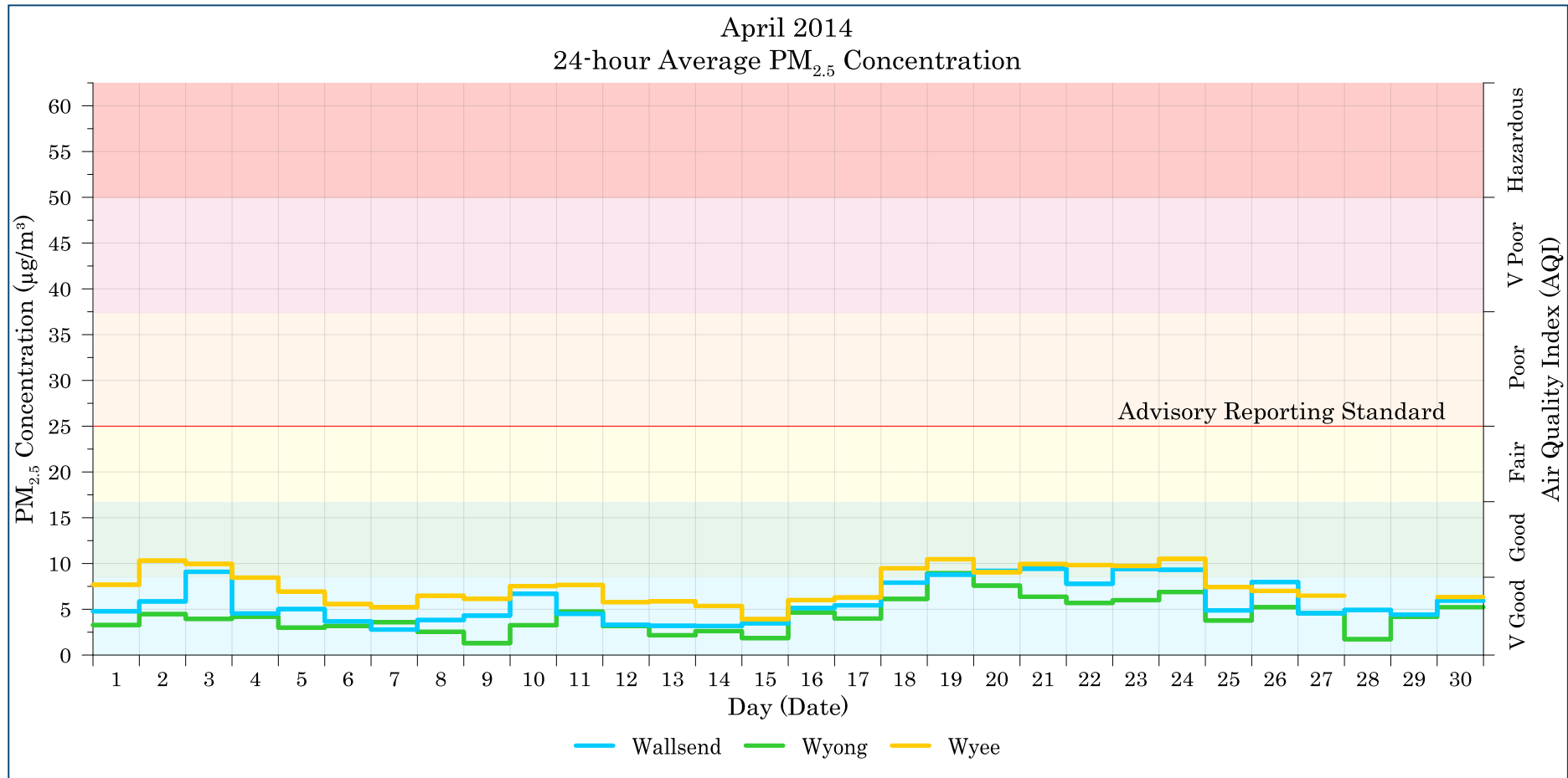
Figure 7-2: Lake Macquarie - Wyong 24-hour average PM 2.5 levels – April 2014
