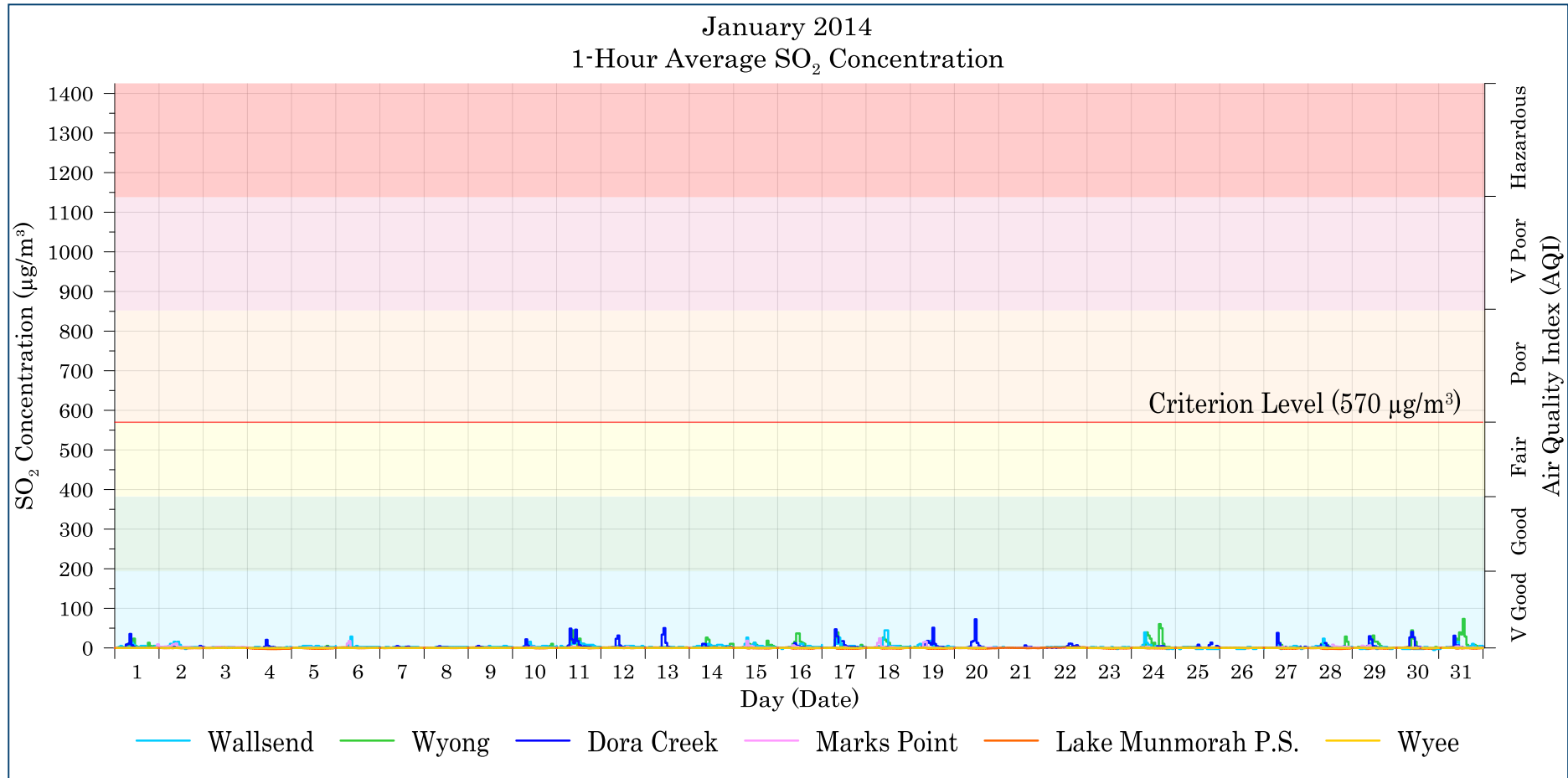
Figure 7-4: Lake Macquarie - Wyong 1-hour average SO 2 levels – January 2014
