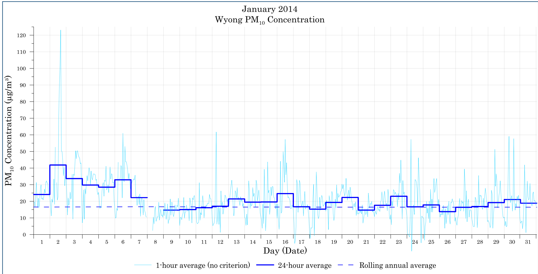
Figure B-2: Wyong PM 10 concentration - January
