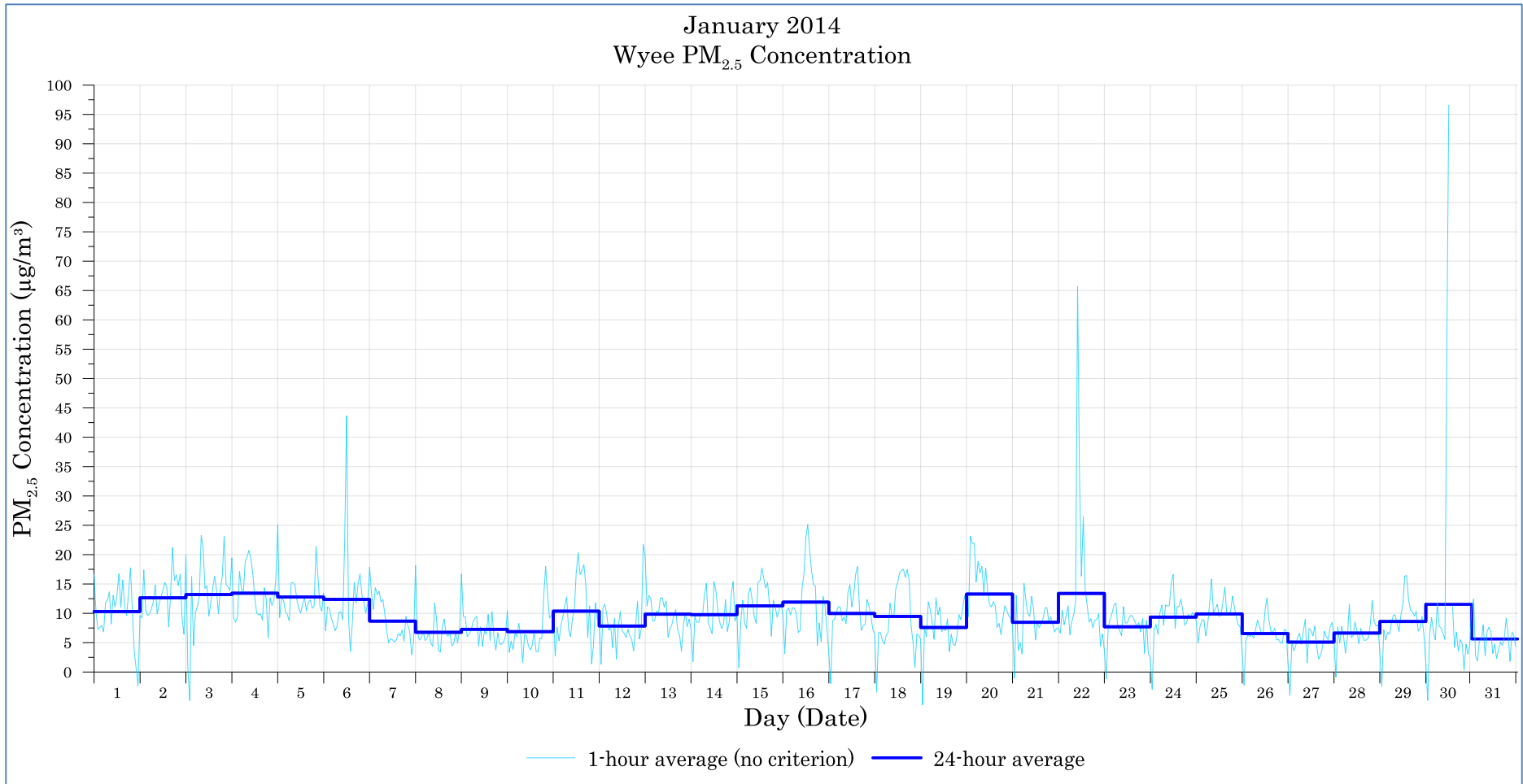
Figure B-5: Wyee PM 2.5 concentration - January
