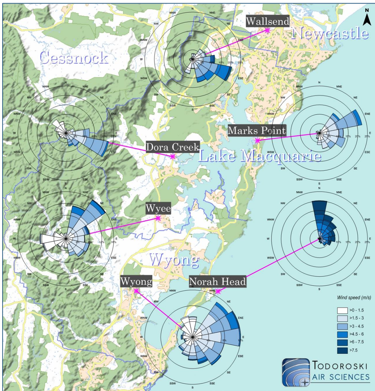
Figure 6-1: January windroses – Wallsend, Dora Creek, Marks Point, Wyee, Norah Head and Wyong
