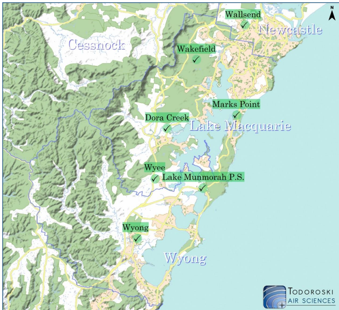
Lake Macquarie – Wyong Air Quality Tabular Summary - January 2014
