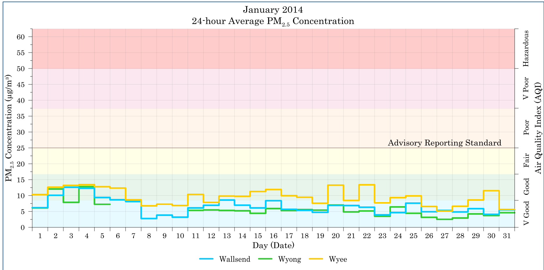
Figure 7-2: Lake Macquarie - Wyong 24-hour average PM 2.5 levels – January 2014
