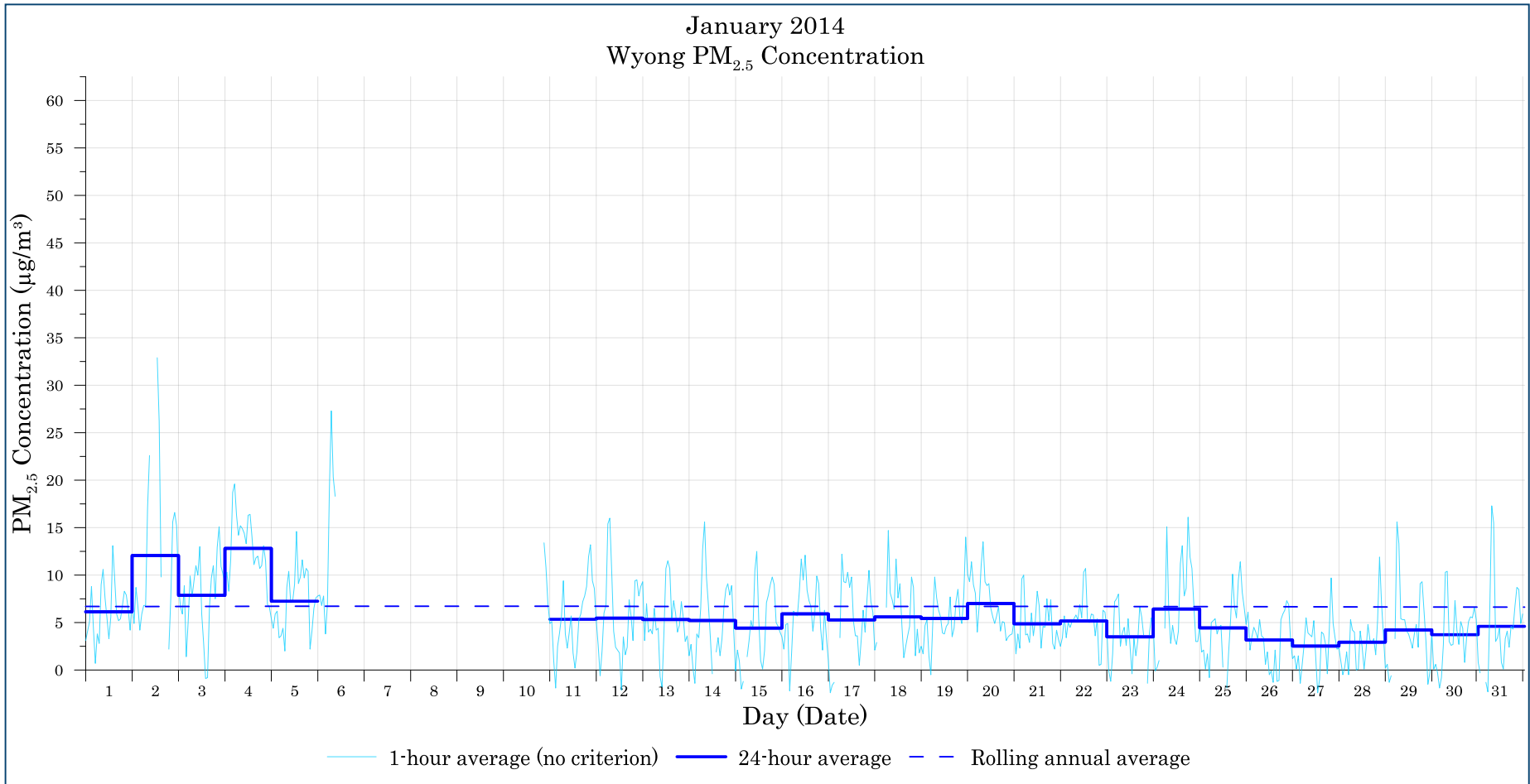
Figure B-4: Wyong PM 2.5 concentration - January
