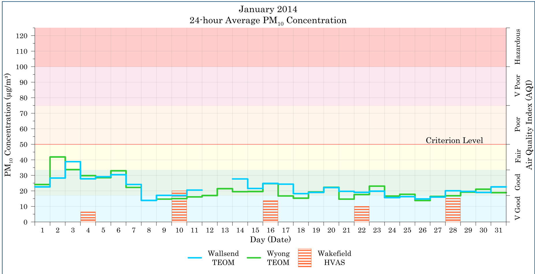
Figure 7-1: Lake Macquarie - Wyong 24-hour average PM 10 levels – January 2014
