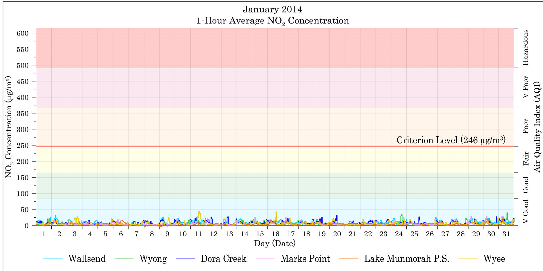
Figure 7-3: Lake Macquarie - Wyong 1-hour average NO 2 levels – January 2014
