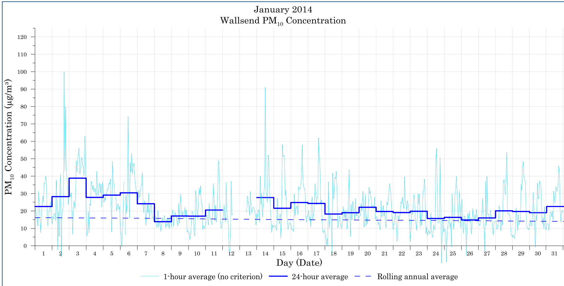
Figure B-1: Wallsend PM 10 concentration - January
