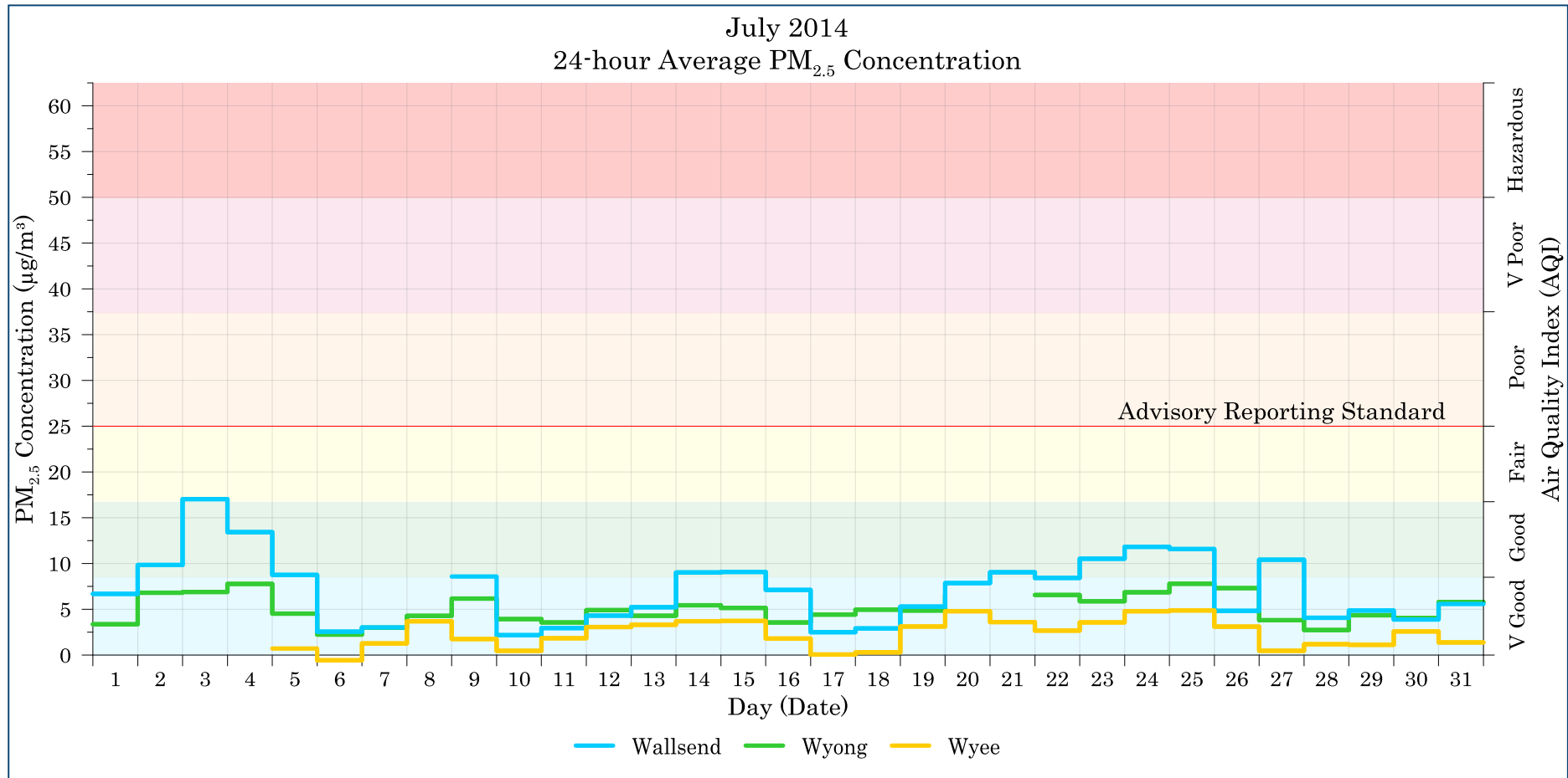
Figure 7-2: Lake Macquarie - Wyong 24-hour average PM 2.5 levels – July 2014
