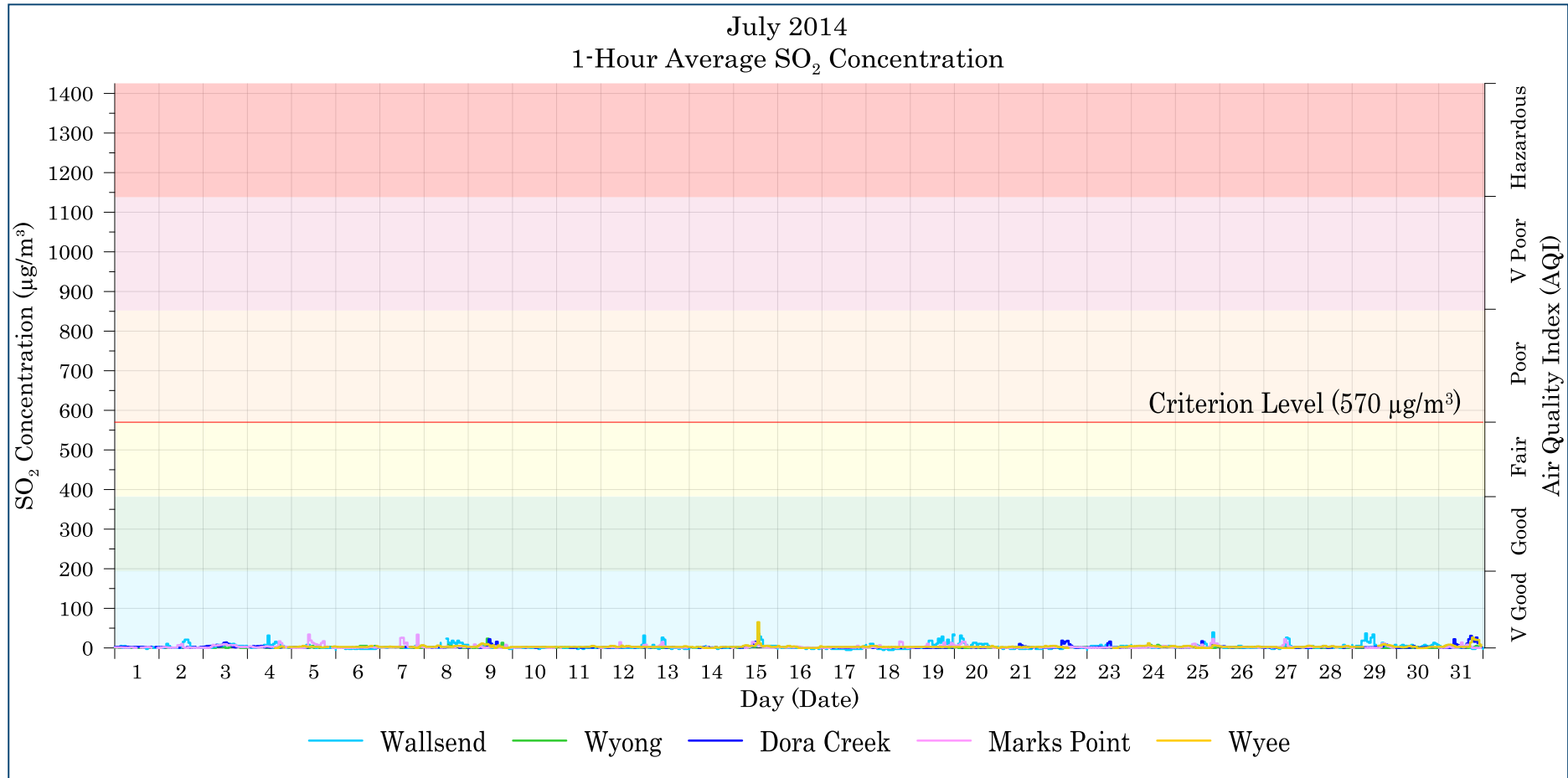
Figure 7-4: Lake Macquarie - Wyong 1-hour average SO 2 levels – July 2014
