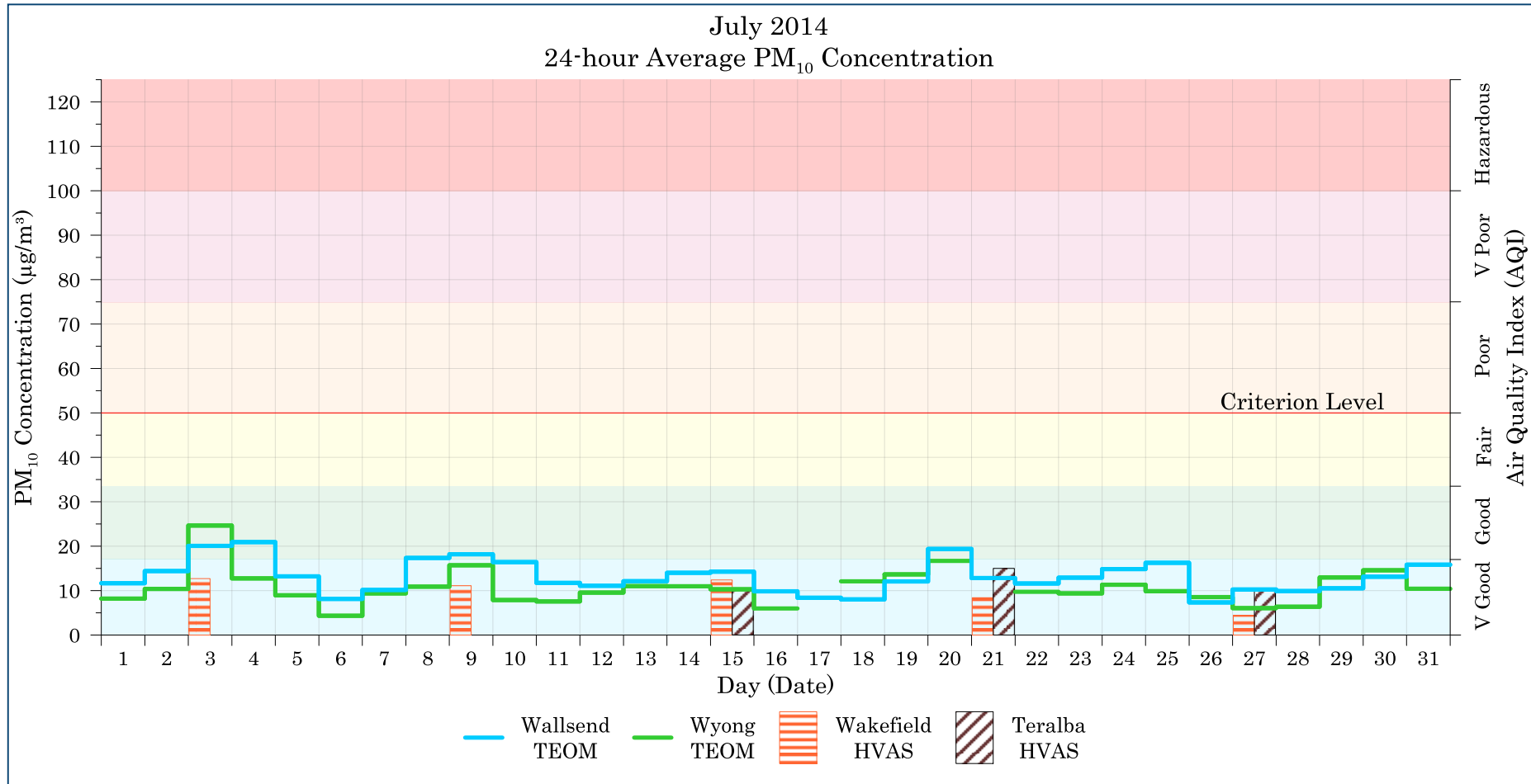
Figure 7-1: Lake Macquarie - Wyong 24-hour average PM 10 levels – July 2014
