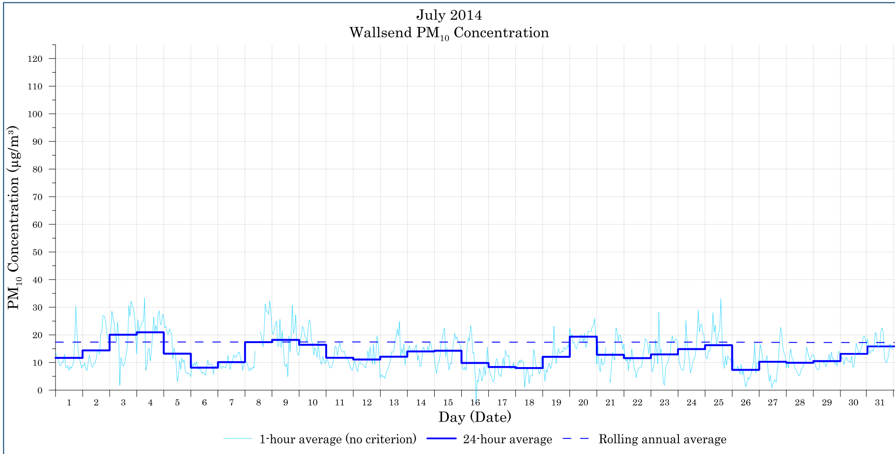
Figure B-1: Wallsend PM 10 concentration - July
