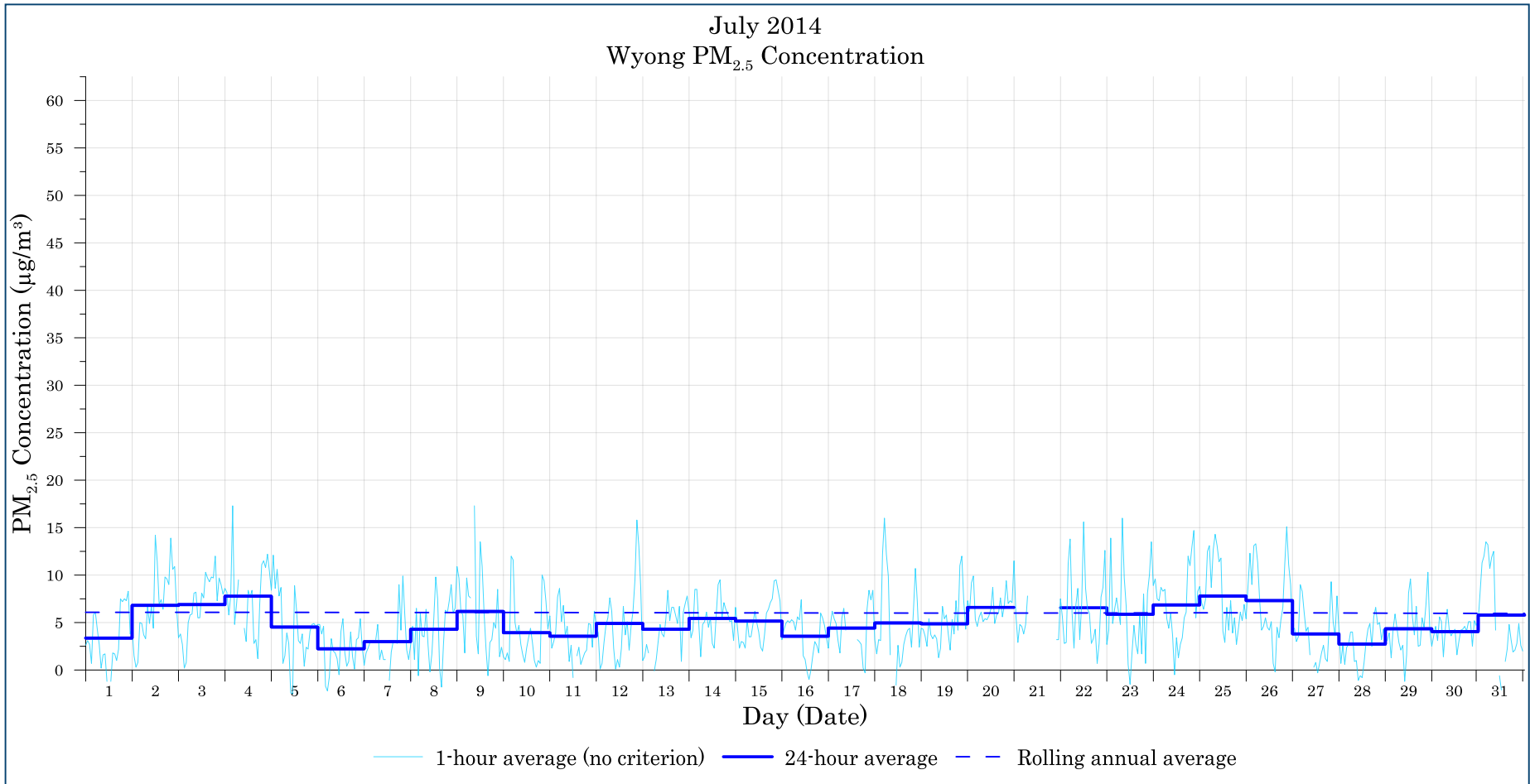
Figure B-4: Wyong PM 2.5 concentration - July
