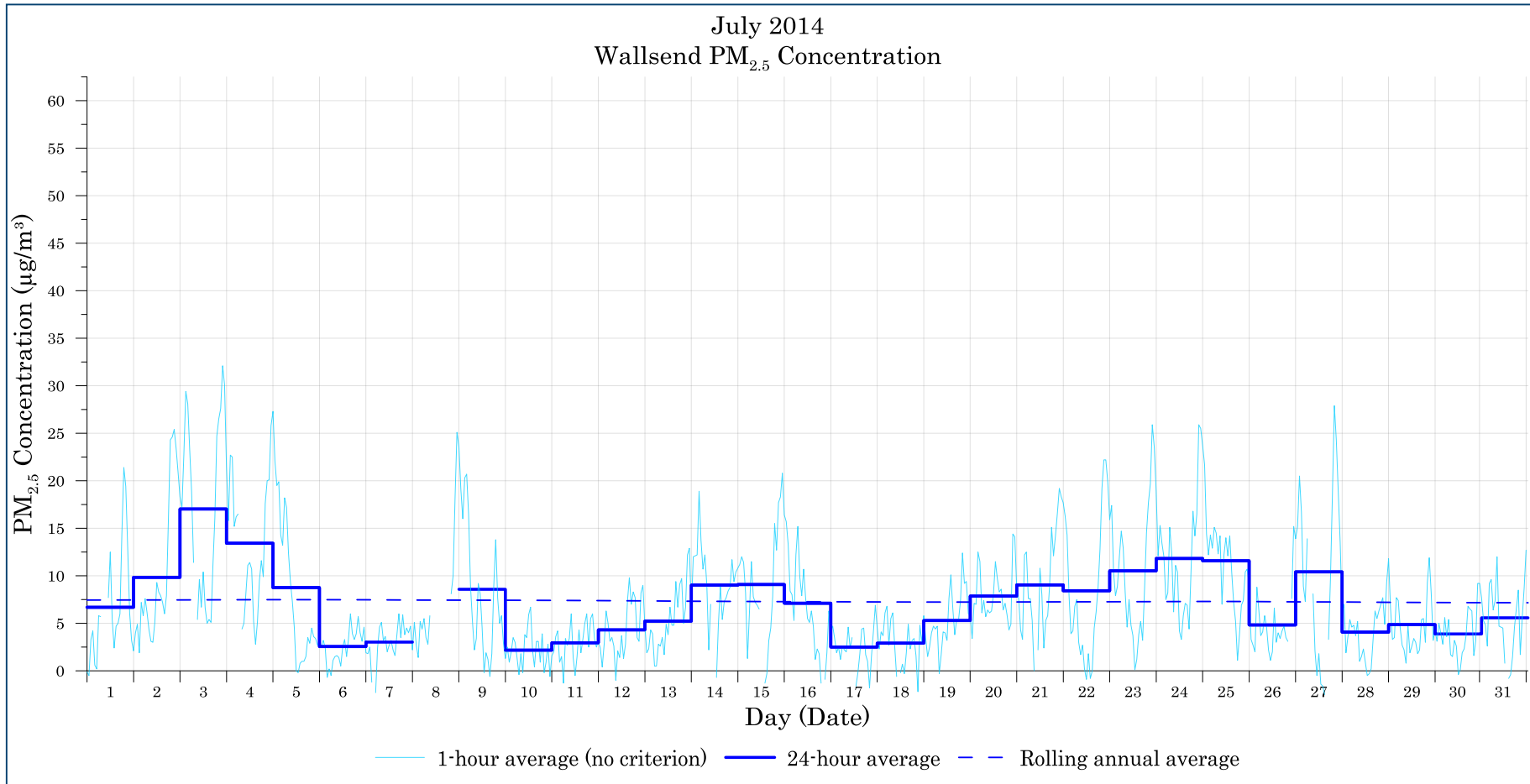
Figure B-3: Wallsend PM 2.5 concentration - July
