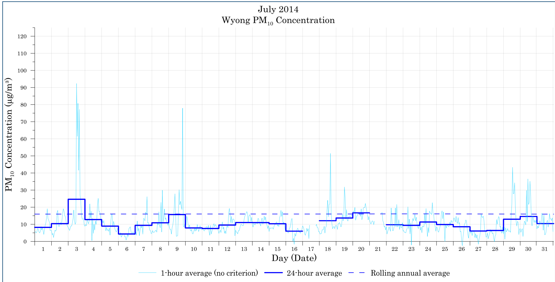
Figure B-2: Wyong PM 10 concentration - July
