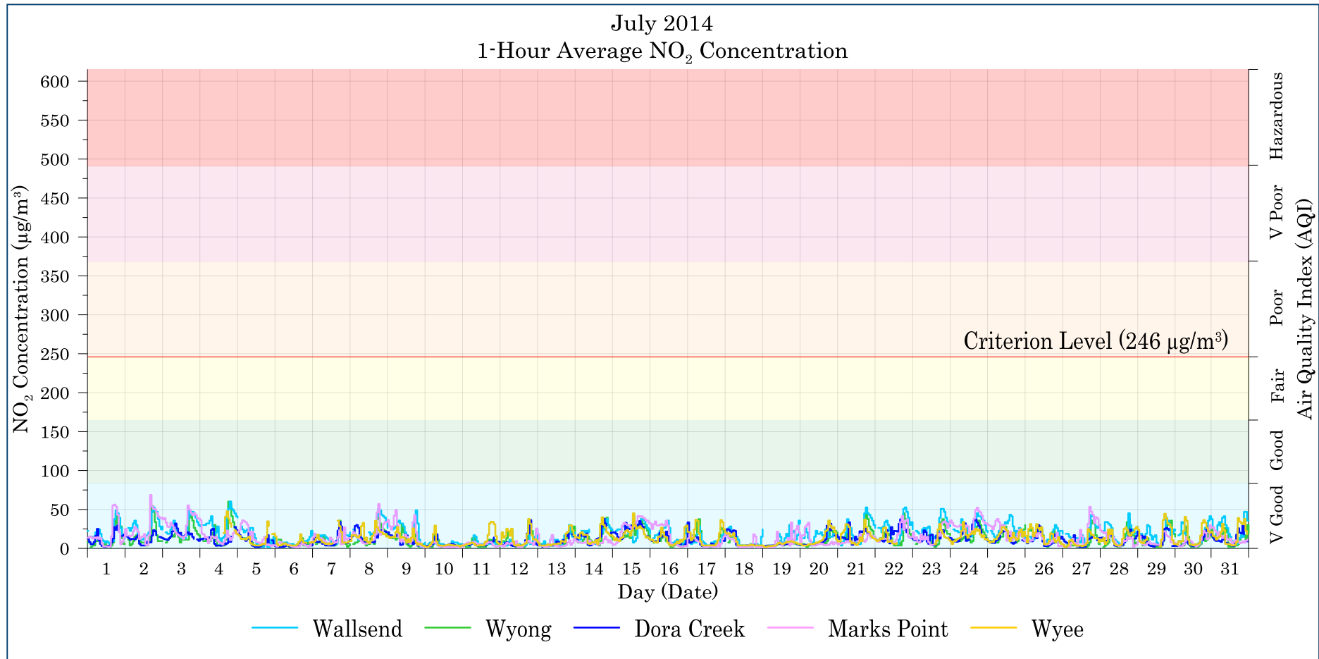
Figure 7-3: Lake Macquarie - Wyong 1-hour average NO 2 levels – July 2014
