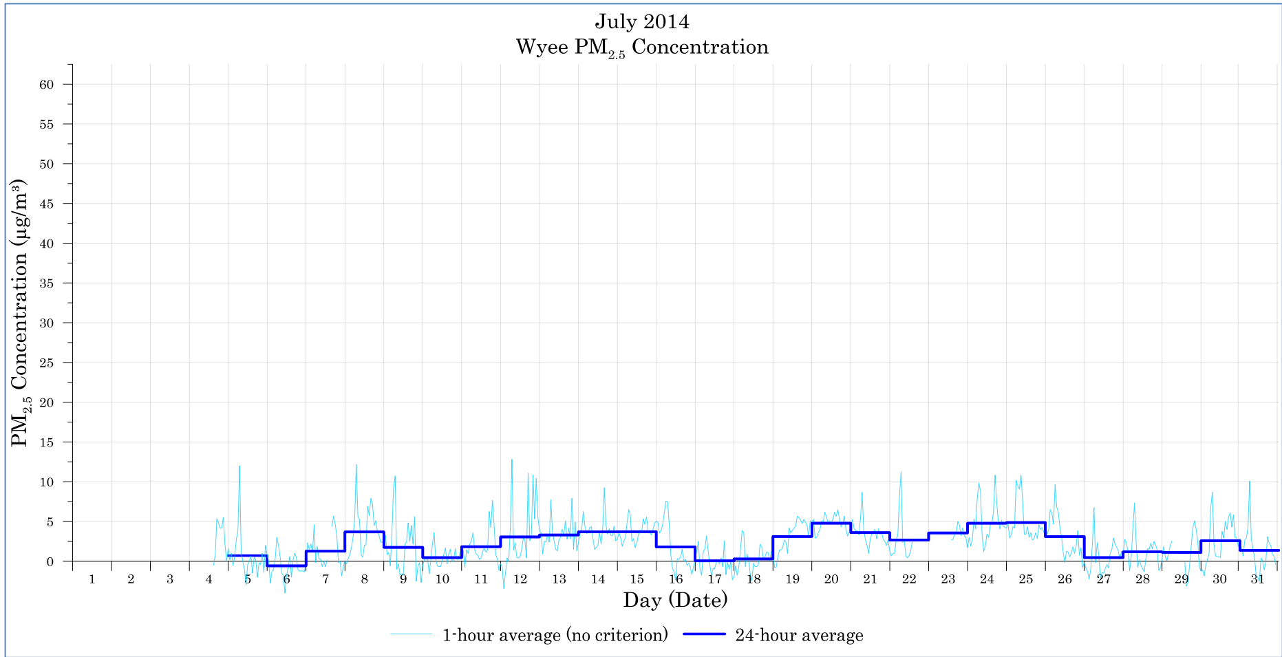
Figure B-5: Wyee PM 2.5 concentration - July
