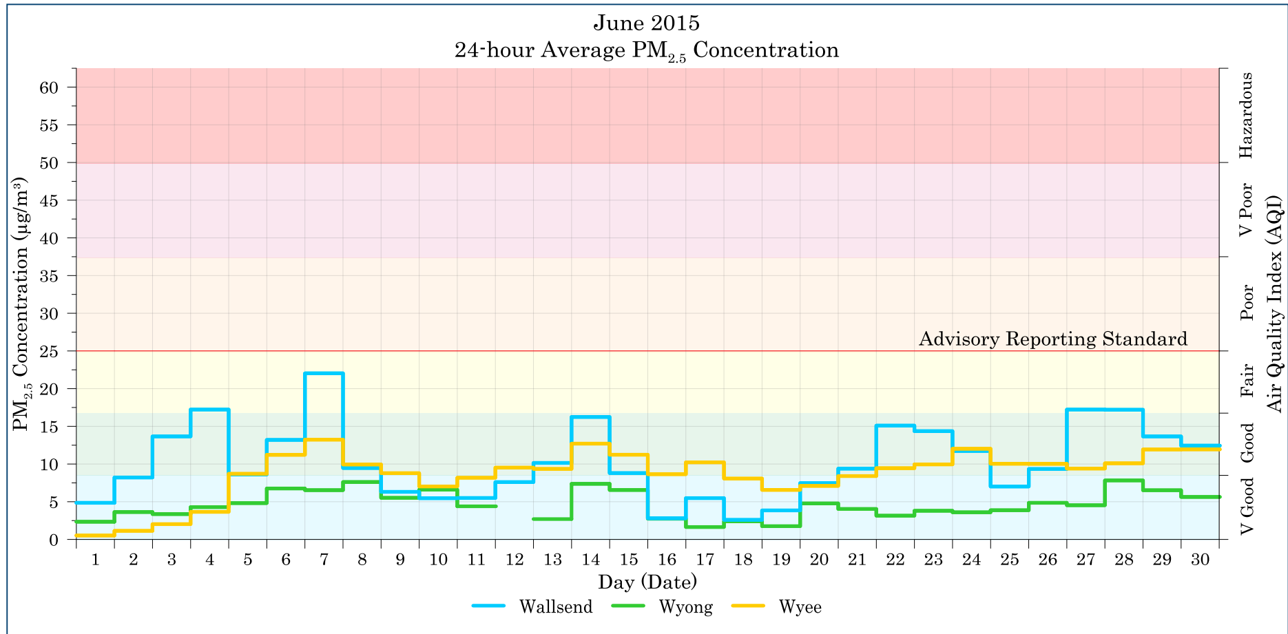
Figure 7-2: Lake Macquarie - Wyong 24-hour average PM 2.5 levels – June 2015
