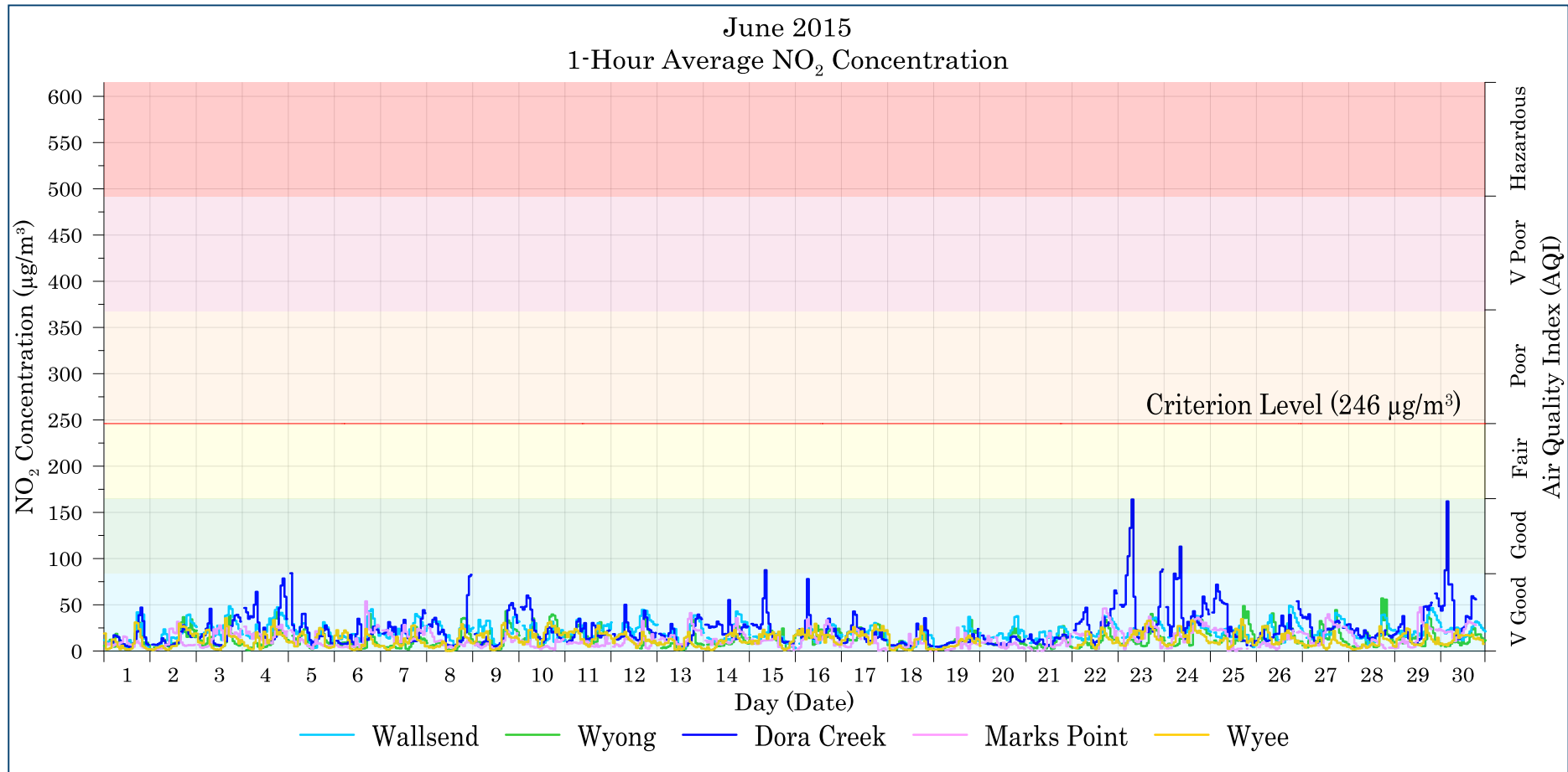
Figure 7-3: Lake Macquarie - Wyong 1-hour average NO 2 levels – June 2015
