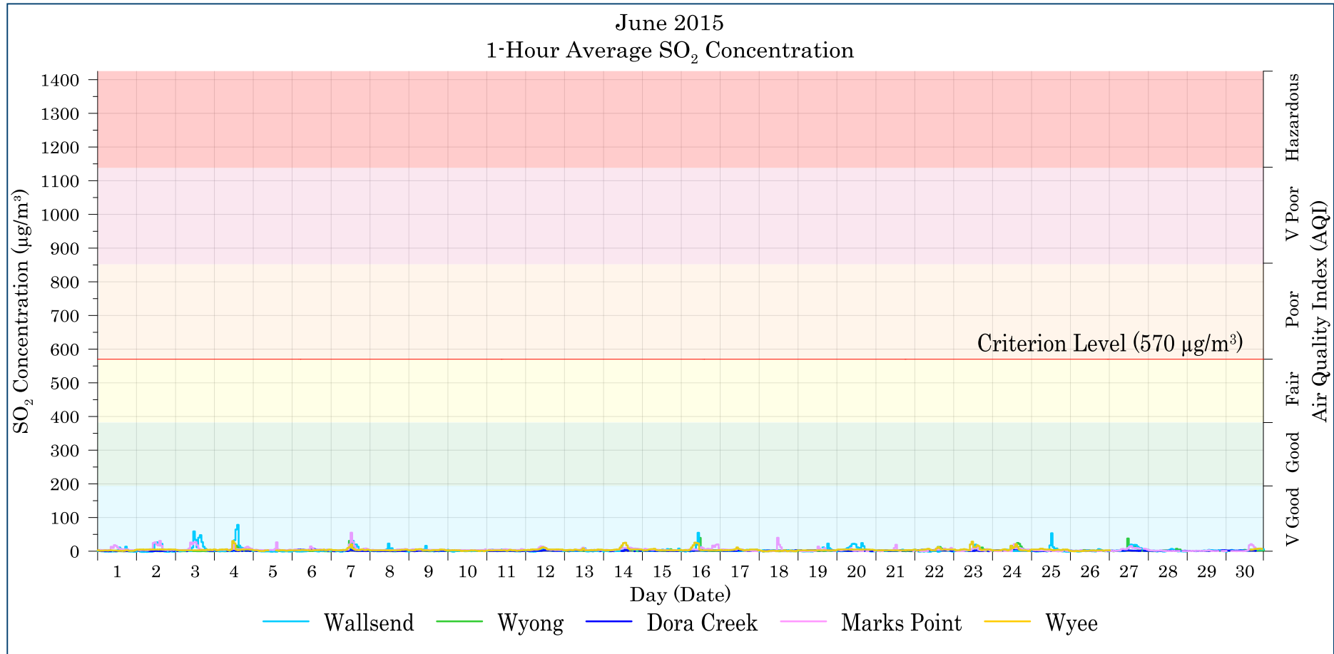
Figure 7-4: Lake Macquarie - Wyong 1-hour average SO 2 levels – June 2015
