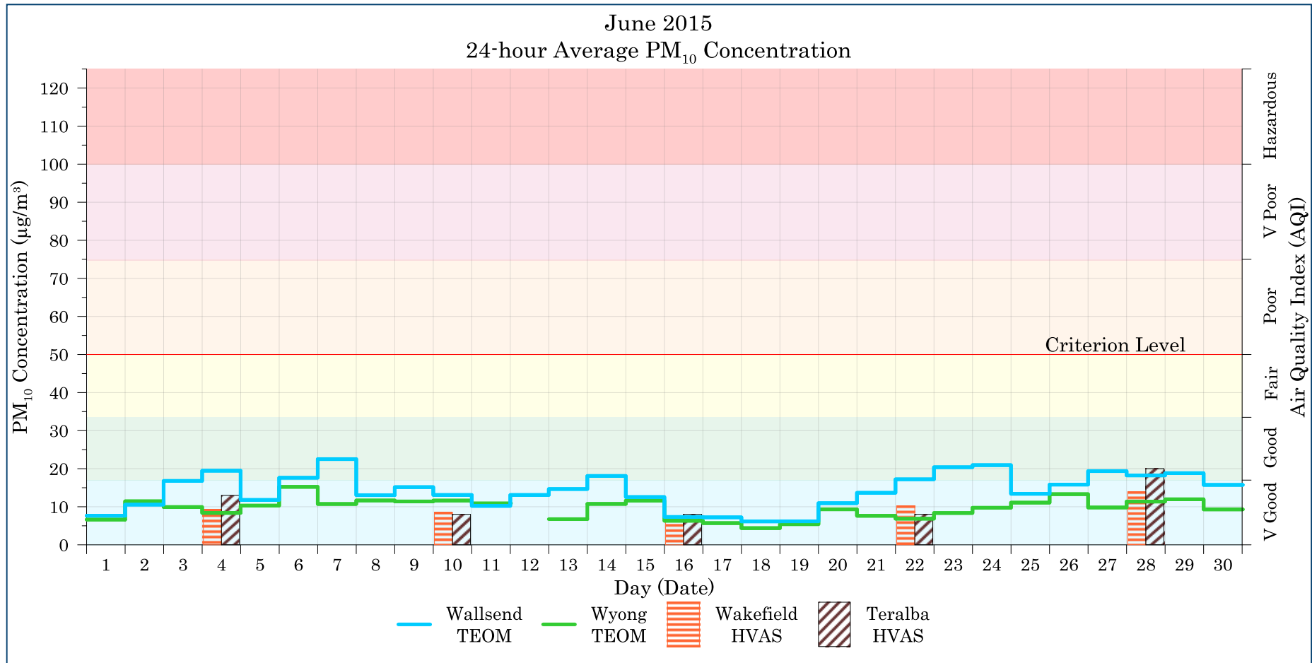
Figure 7-1: Lake Macquarie - Wyong 24-hour average PM 10 levels – June 2015
